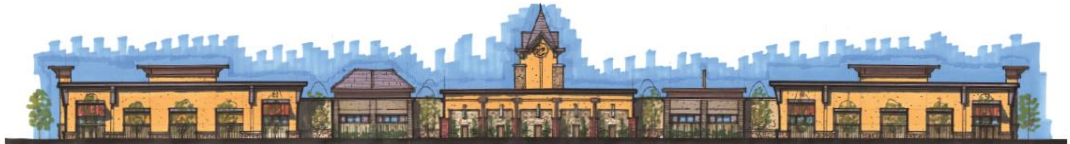
VALLEY VIEW SHOPPE'S REAR ELEVATION
