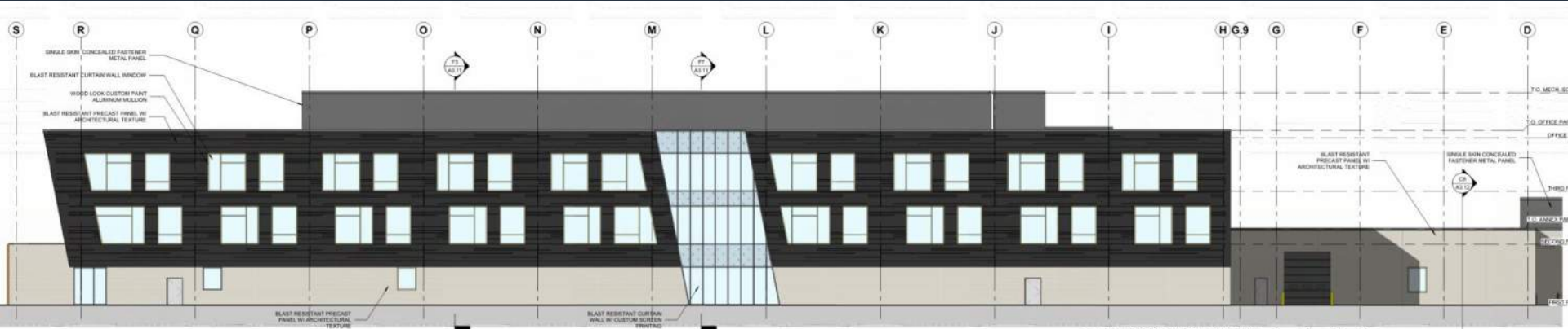
C7 BUILDING - EAST ELEVATION 3/32" = 1'-0"
