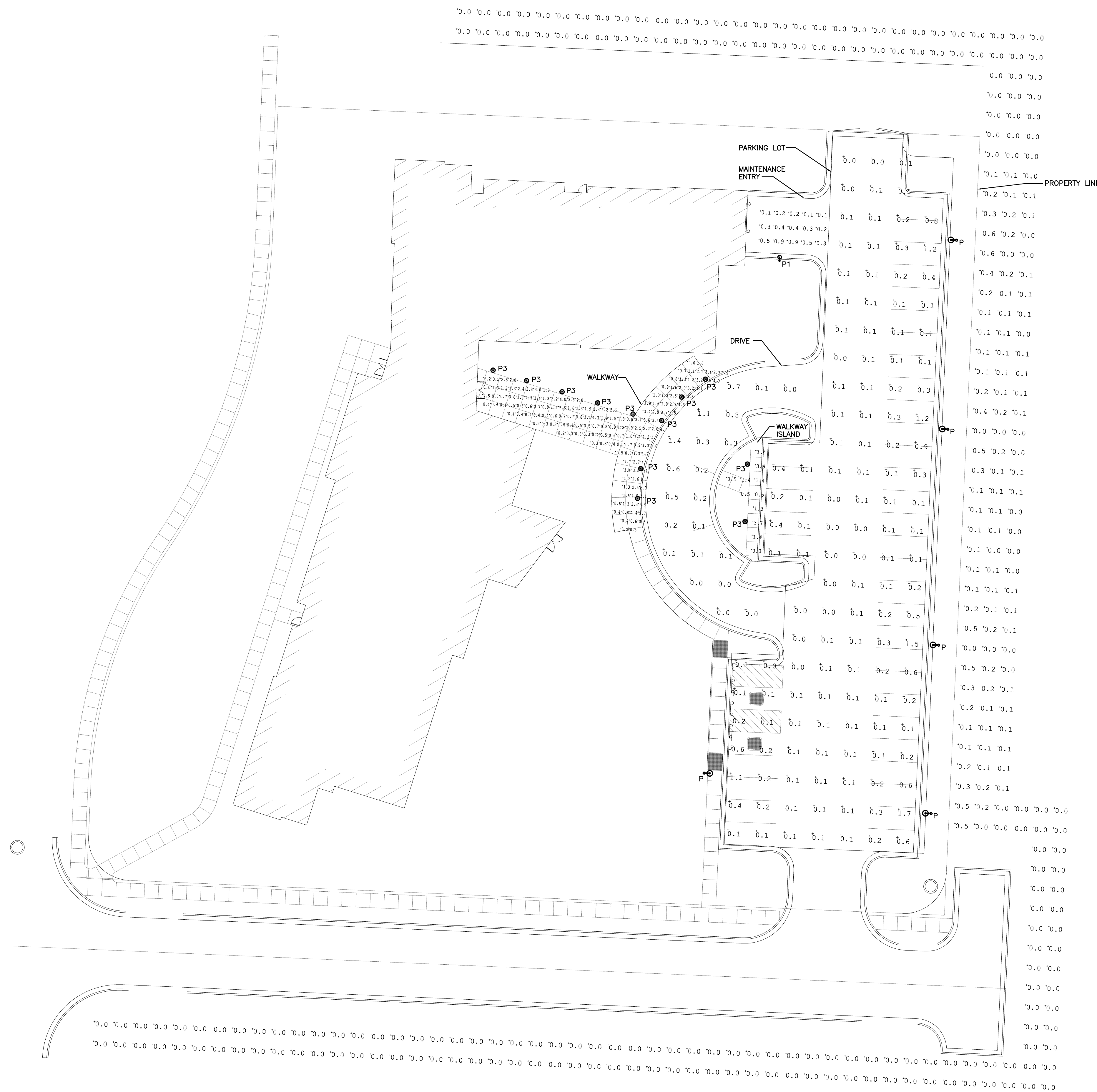
SITE PLAN—PHOTOMETRICS SCALE: 1"=20'-0"
