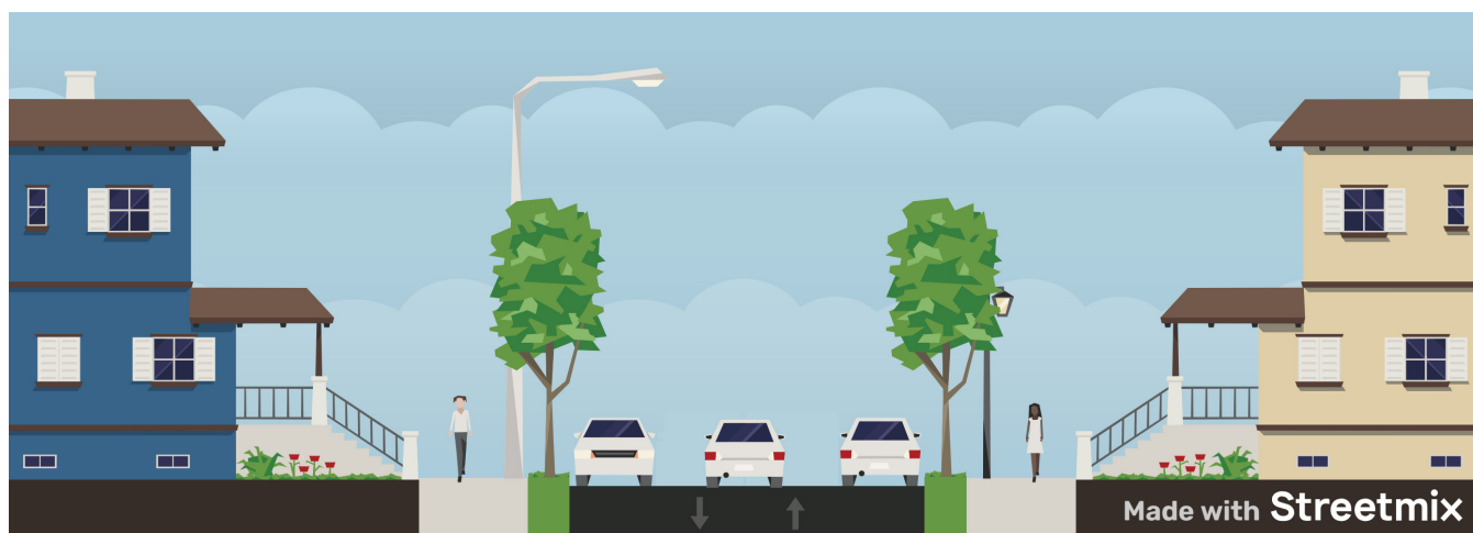
50-foot ROW: Two-way segment with parking permitted on both sides
