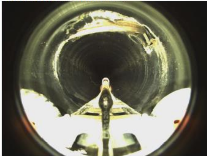
82ft Point of Interest - Pipe damage
