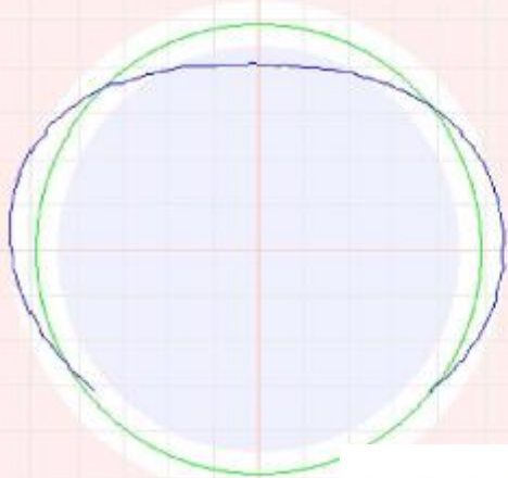
82ft Point of Interest - Pipe damage
