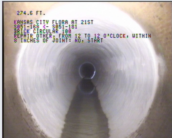
Cementitious Liner Repair of Brick Sewer
