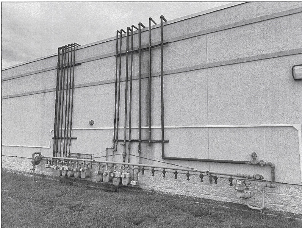
Looking north – rusting/corrosion of gas lines
