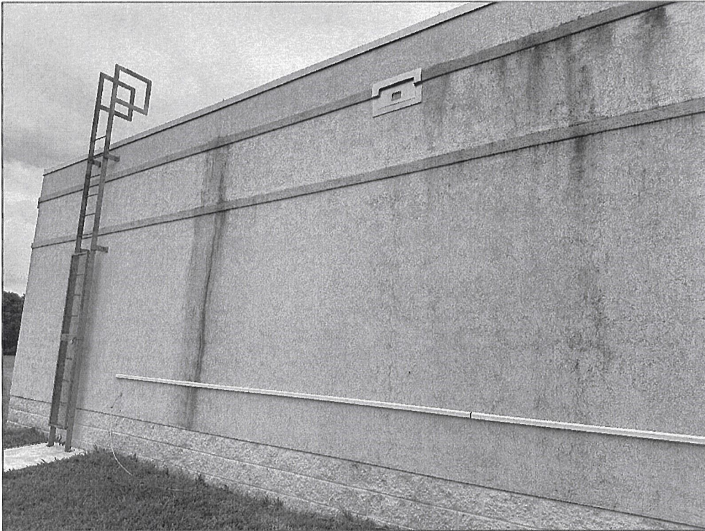
Looking northwest – rusting of ladder/enclosure; water damage to EIFS; failure of finishes
