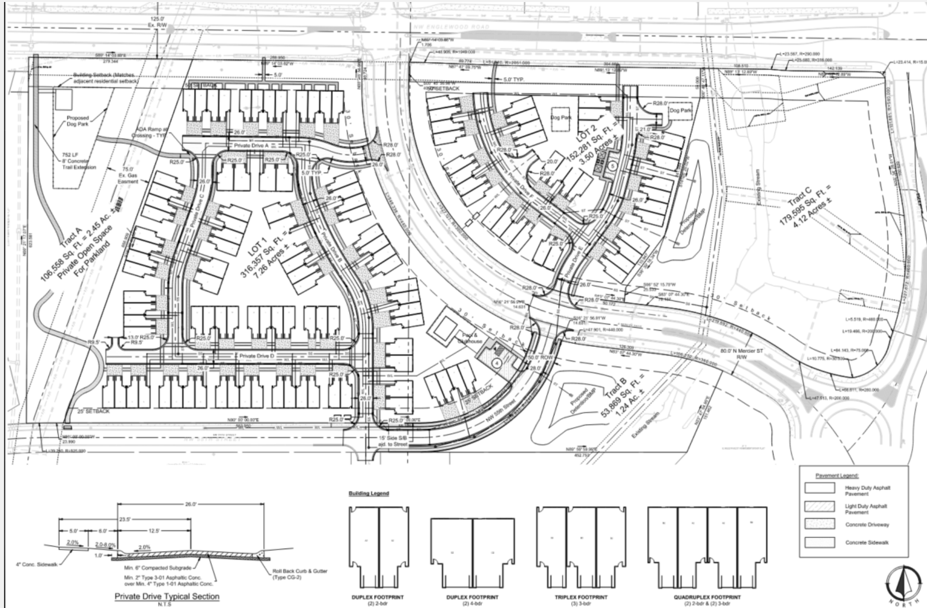
Site Plan
