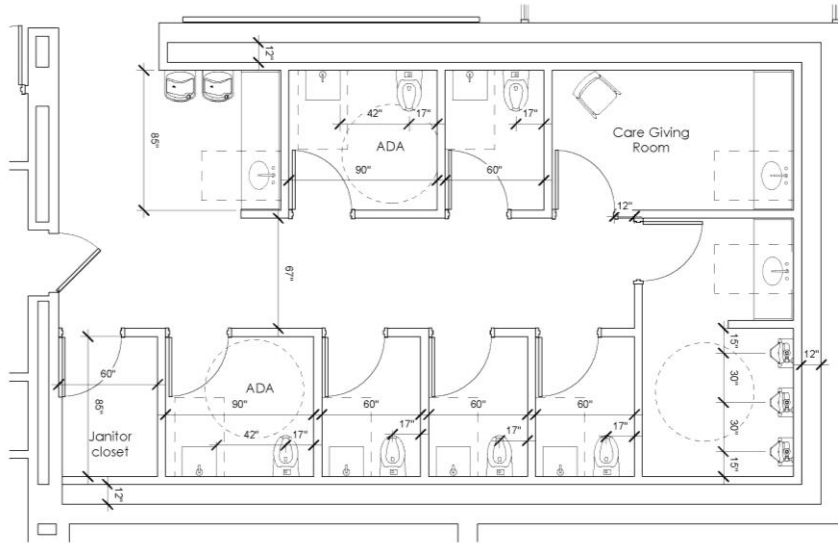
Proposed All Gender Restroom Layout Design and Representation
