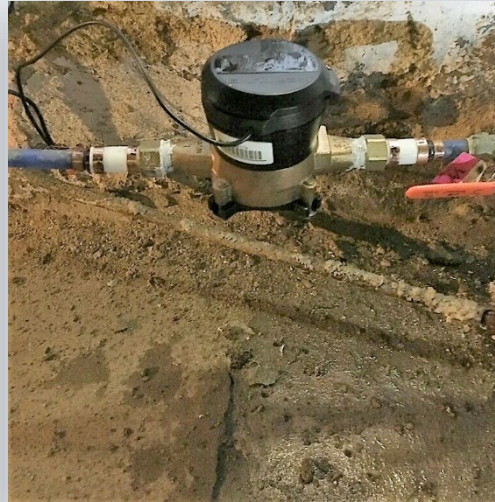
Automated Metering Equipment and Installation
