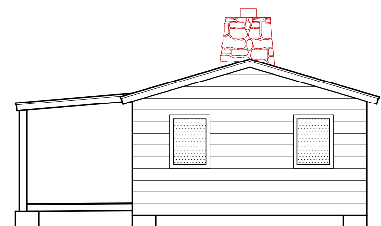
BLDG 2 - RIGHT SIDE ELEVATION 1/16" = 1'-0"
