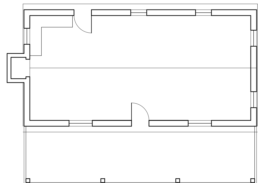
BLDG 2 - CABIN PLAN 1/16" = 1'-0"
