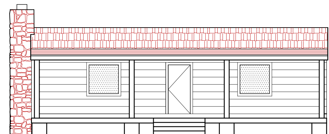
BLDG 2 - FRONT ELEVATION 1/16" = 1'-0"
