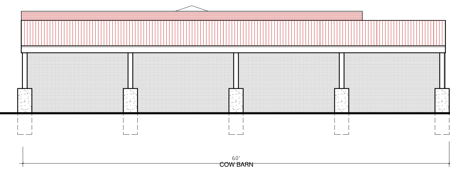
BLDG 2 - FRONT ELEVATION 1" = 20'-0"
