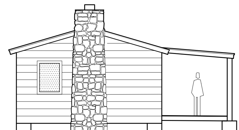
BLDG 2 - LEFT SIDE ELEVATION 1/16" = 1'-0"
