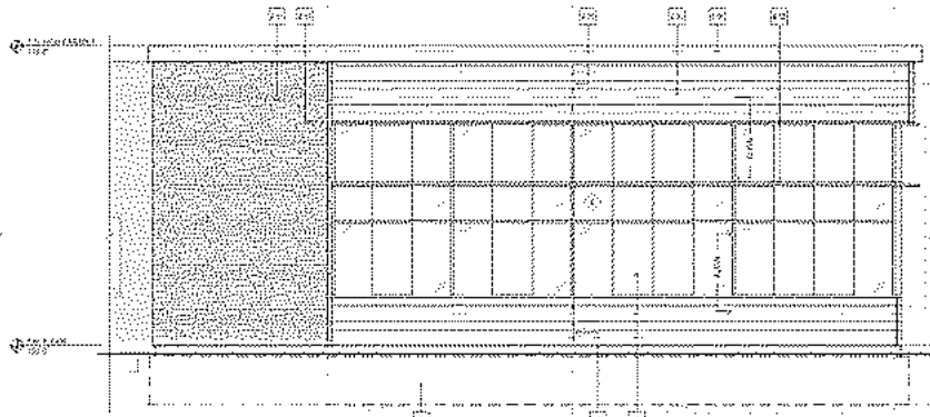
SOUTHEAST ELEVATION SOUTHEAST SIDE - 11' x 12'
