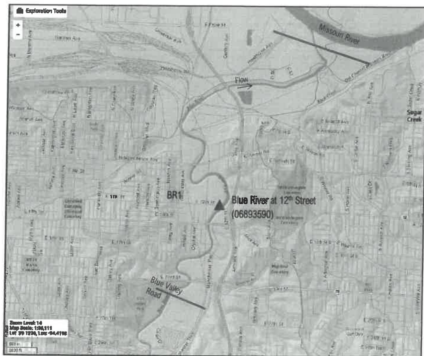
Figure 2. Blue River Reach 1 (BR1), extending 5.7 miles downstream from the upstream model boundary near northern Blue Valley Park Road at Blue Valley Park, through the USGS gaging station at 12 th Street, downstream to a location near the confluence with the Missouri River.
